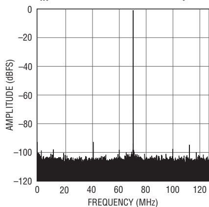
LTC2157-12: 32K Point FFT, f_{IN} = 70\text{MHz} , -1dBFS, 250Mps
