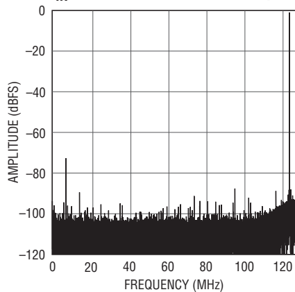
LTC2157-12: 32K Point FFT, f_{IN} = 380\text{MHz} , -1dBFS, 250Mps
