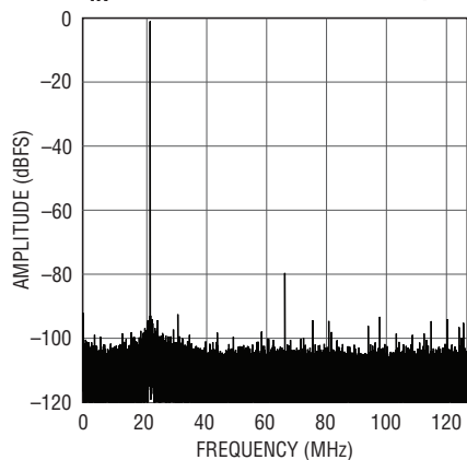
LTC2157-12: 32K Point FFT, f_{IN} = 229\text{MHz} , -1dBFS, 250Mps
