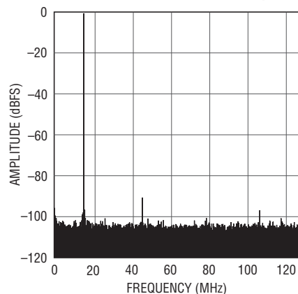
LTC2157-12: 32K Point FFT, f_{IN} = 15\text{MHz} , -1dBFS, 250Mps
