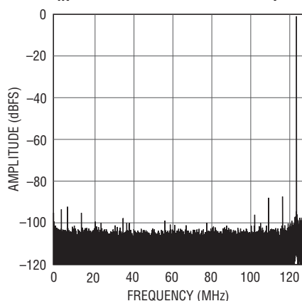
LTC2157-12: 32K Point FFT, f_{IN} = 122\text{MHz} , -1dBFS, 250Mps
