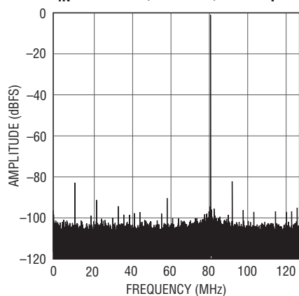
LTC2157-12: 32K Point FFT, f_{IN} = 171\text{MHz} , -1dBFS, 250Mps
