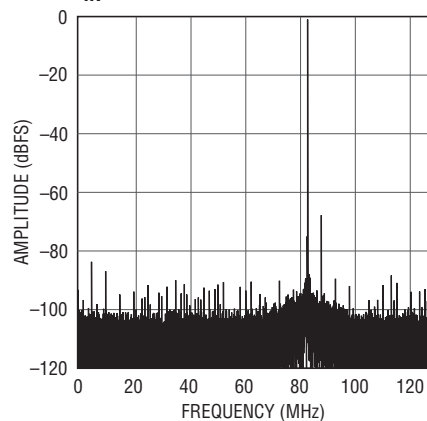
LTC2157-12: 32K Point FFT, f_{IN} = 420\text{MHz} , -1dBFS, 250MHz
