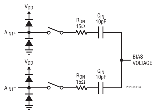
Figure 3. The Equivalent Circuit for the Differential Analog Input of the LTC2323-14
