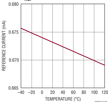
I_{REF} vs Temperature, V_{REF} = 4.096\text{V}
