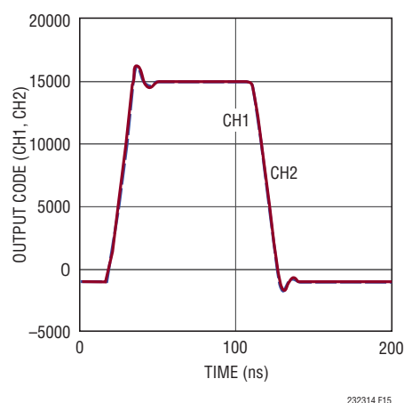
Figure 15. Transient Response of the LTC2323-14
