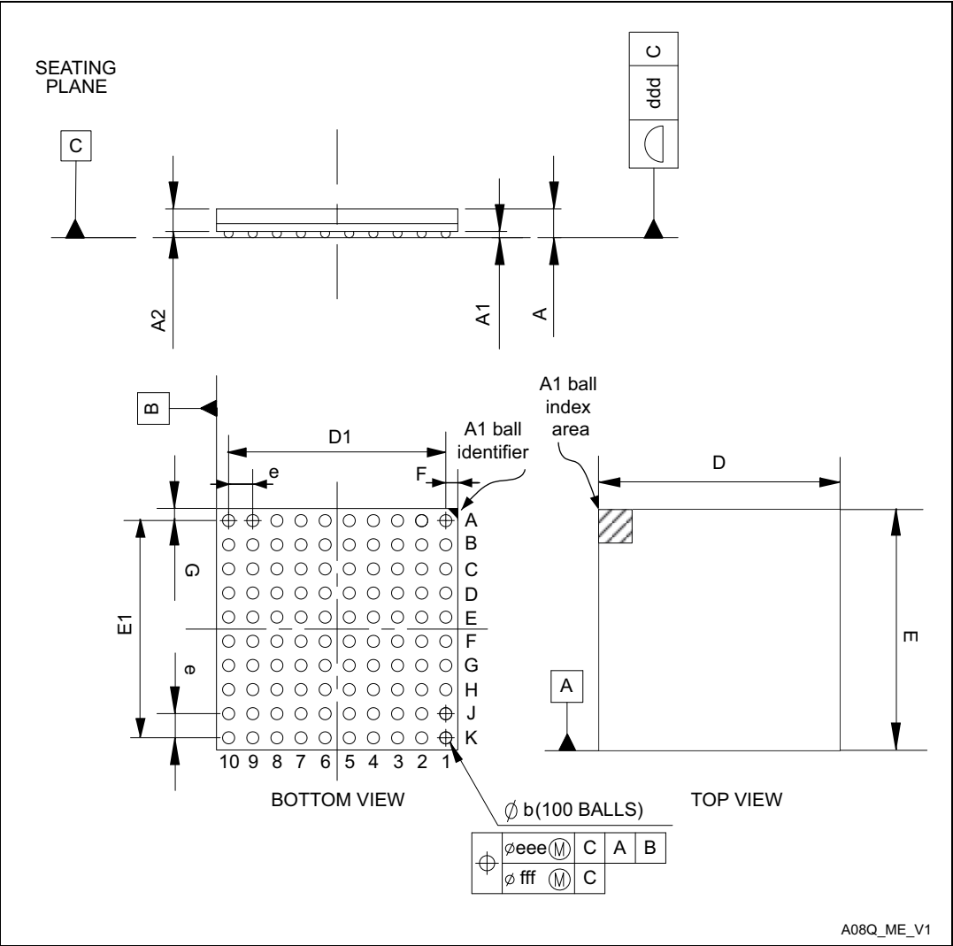
Figure 79. TFBGA100 - Outline
