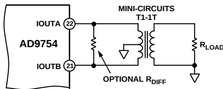
Figure 27. Differential Output Using a Transformer
