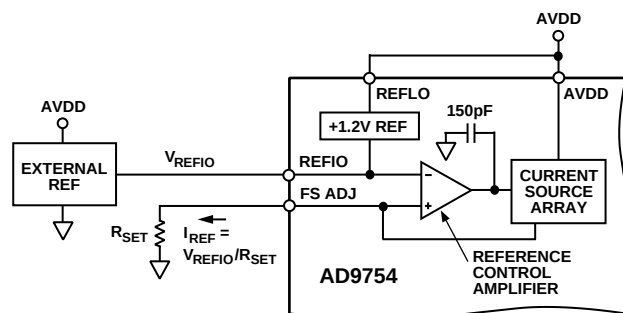
Figure 18. External Reference Configuration
