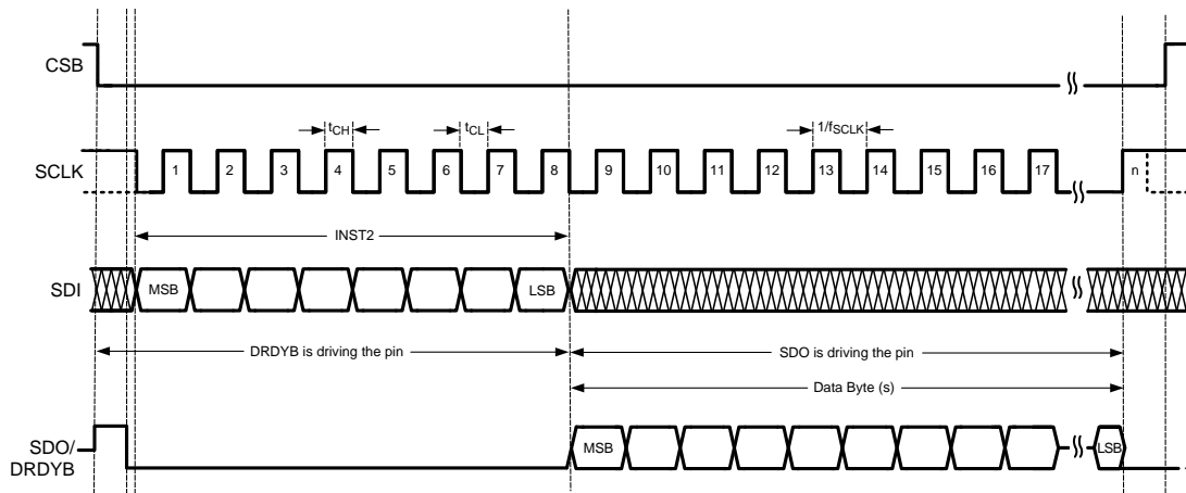
Figure 1. Timing Diagram
