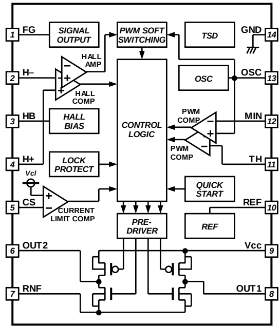
Fig.2 Block diagram
