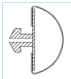
UNIVERSAL MOUNTING
