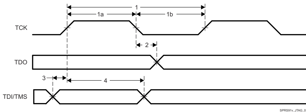
Figure 8-19. JTAG Timing
