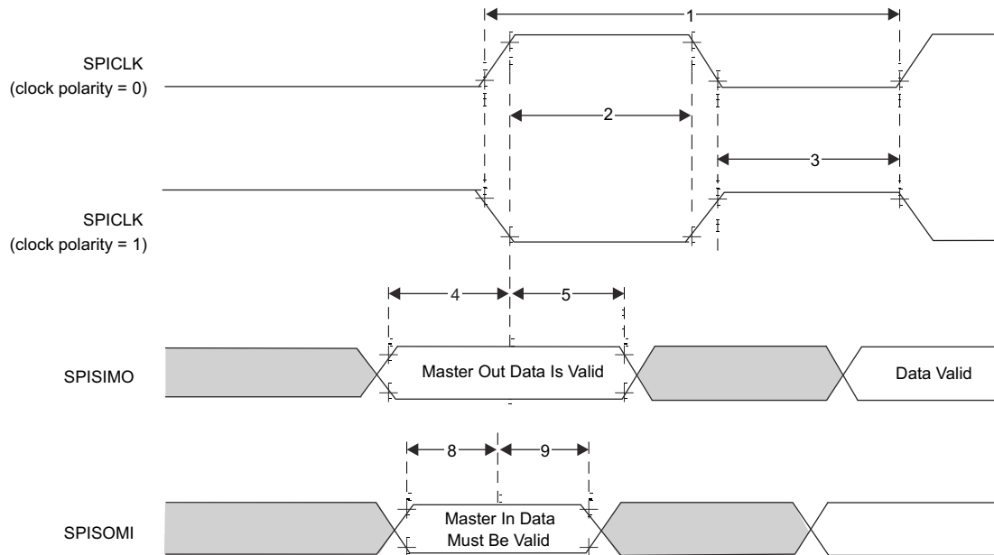
Figure 8-5. SPI Master Mode External Timing (CLOCK PHASE = 1)
