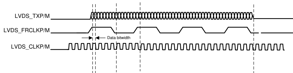
Figure 8-10. LVDS Interface Lane Configuration And Relative Timings
