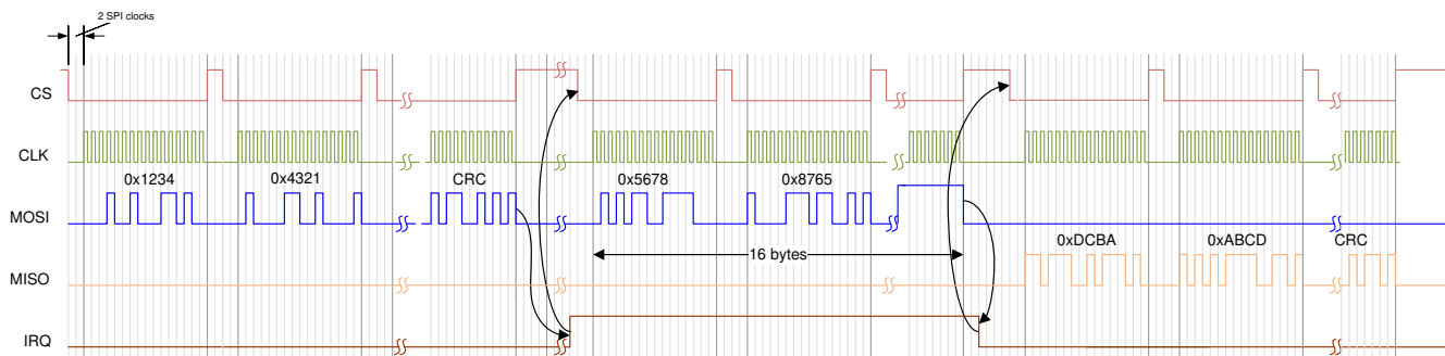
Figure 8-9. SPI Communication
