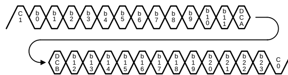
Figure 25. Channel Link II Serial Stream (DS92LV042x)
