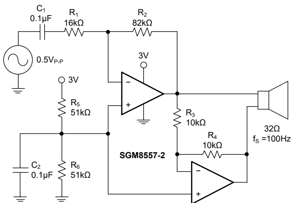
Figure 2. 200mW Bridge Amplifier at 3V
