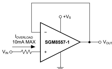
Figure 4. Input Current-Limit Protection
