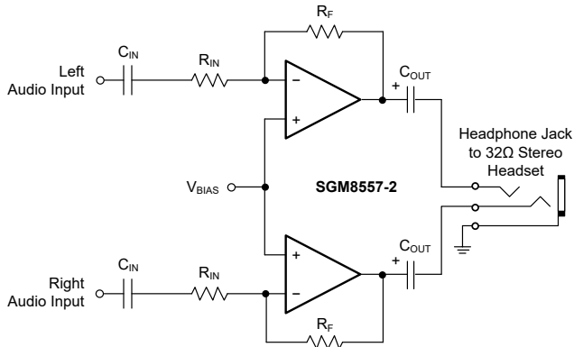
Figure 1. Stereo Headphone Driver
