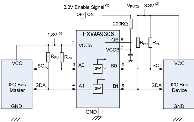
Figure 6. Application (Switch Enable Control)
