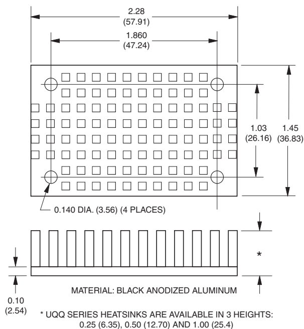
Dimensions in inches (mm) Figure 8. Optional Heatsink
