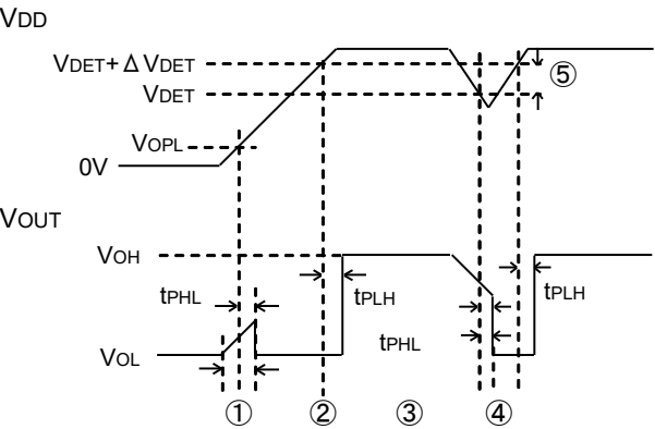
Fig. 14 Timing Waveforms
