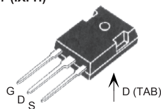
TO-247 (IXFH)
