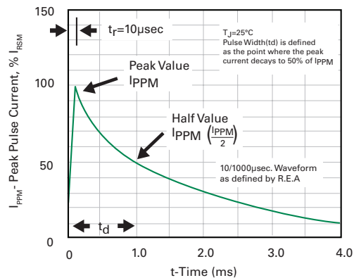
Figure 4 - Pulse Waveform
