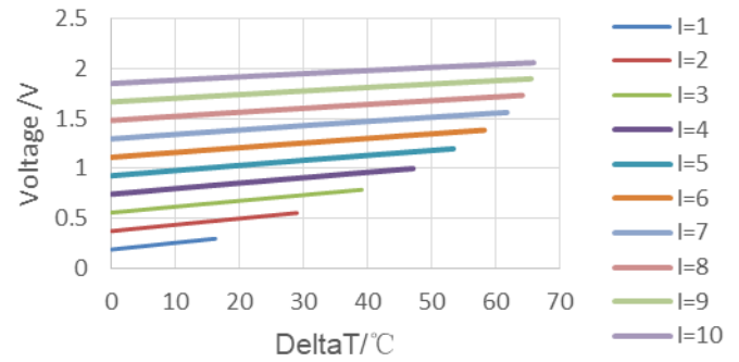
Performance Curves at T_h=27^\circ\text{C}
