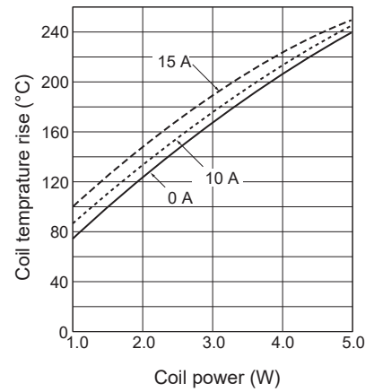
Operating Coil temperature rise
