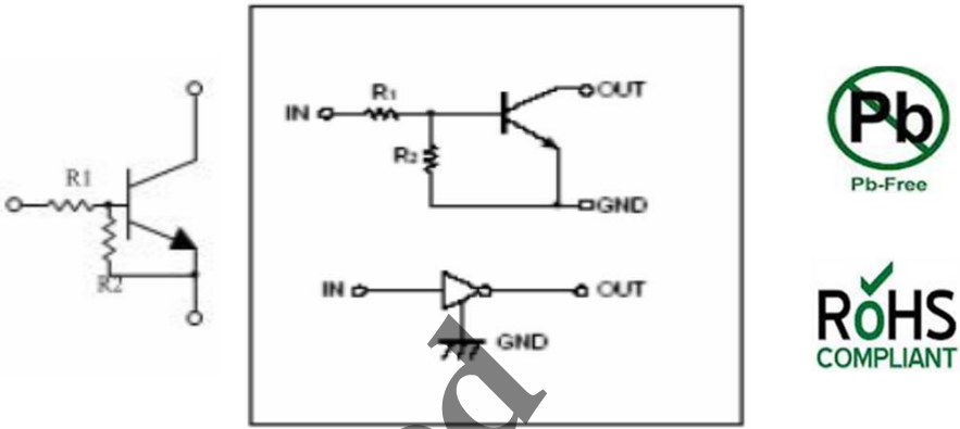
Equivalent Circuit
