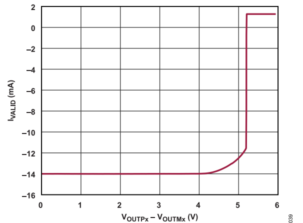
Figure 39. I_{INVALID} vs. V_{OUTPx} - V_{OUTMx}
