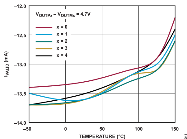
Figure 41. I_{\text{INVALID}} vs. Temperature, V_{\text{OUTPx}} - V_{\text{OUTMx}} = 4.7\text{V}
