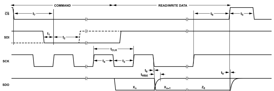
Figure 2. SPI Bus Timing Diagram
