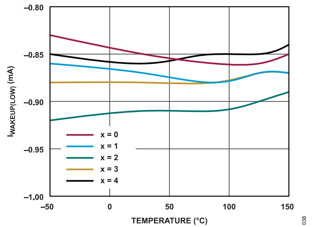
Figure 38. I_{WAKEUP(LOW)} vs. Temperature
