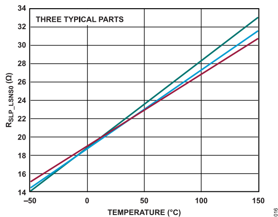
Figure 16. R_{SLP\_LSN0} vs. Temperature
