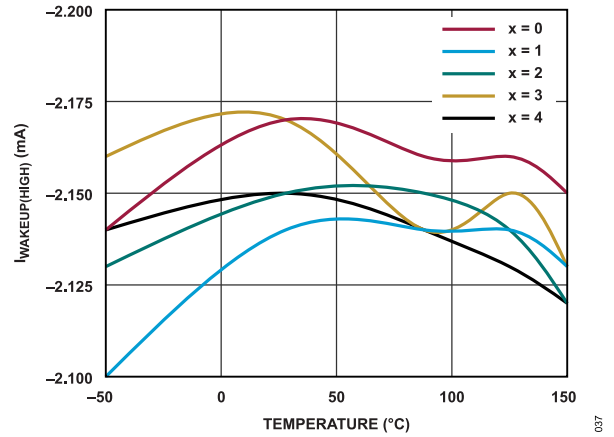
Figure 37. I_{WAKEUP(HIGH)} vs. Temperature
