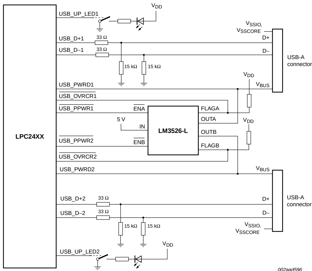
Fig 28. LPC2420/2460 USB OTG port configuration: USB port 1 host, USB port 2 host
