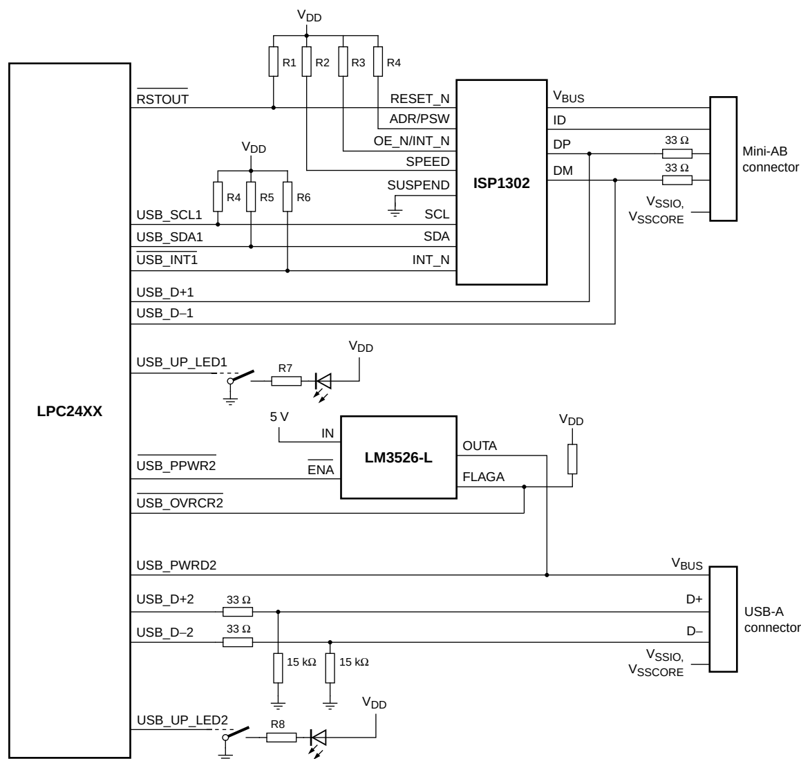
Fig 25. LPC2420/2460 USB OTG port configuration: USB port 1 OTG dual-role device, USB port 2 host
