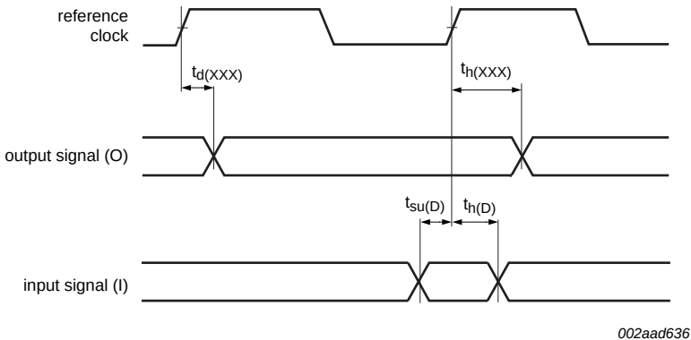
Fig 18. Signal timing
