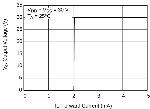
Figure 18. Transfer Characteristics
