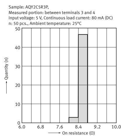
16-5. On resistance distribution
