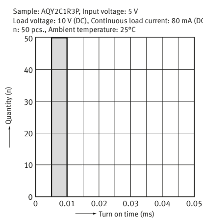
17-4. Turn on time distribution
