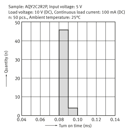
17-3. Turn on time distribution
