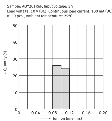
17-1. Turn on time distribution
