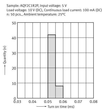
17-2. Turn on time distribution
