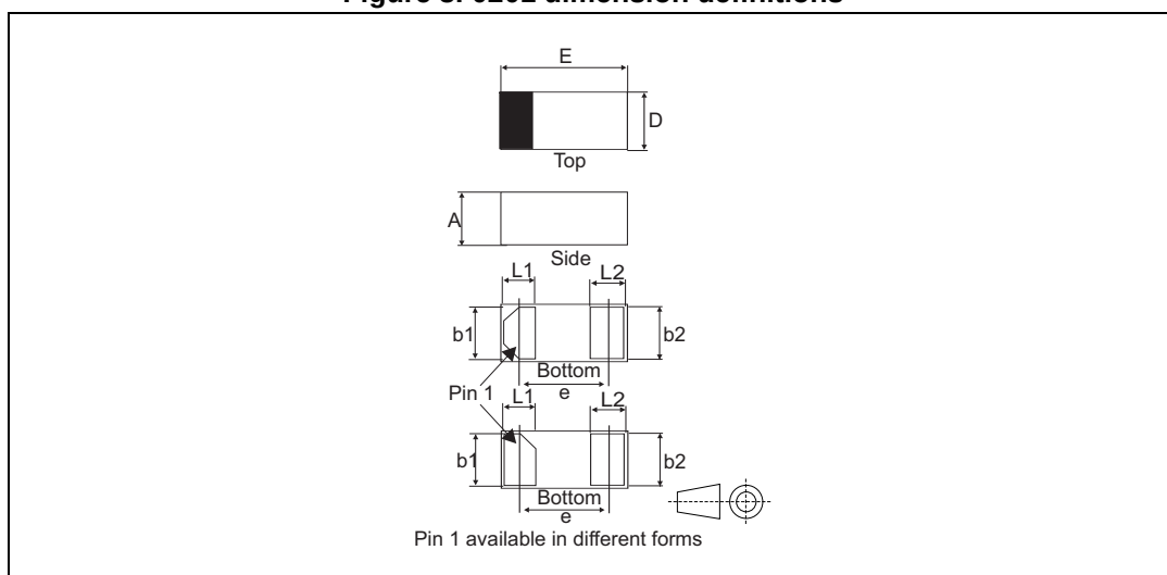
Figure 8. 0201 dimension definitions
