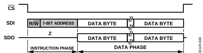
Figure 71. SPI Transaction Phases
