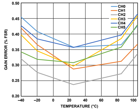
Figure 32. Gain Error vs. Temperature
