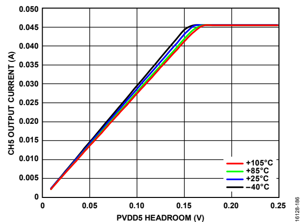
Figure 46. CH5 Output Current vs. PVDD5 Headroom for Various Temperatures
