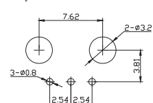
PCB Layout for Electrical Circuit
