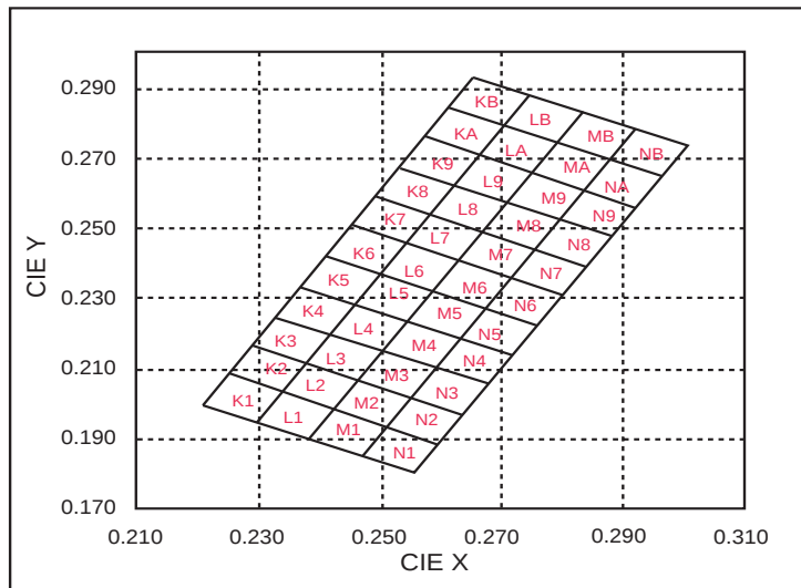
Chromaticity Diagram
