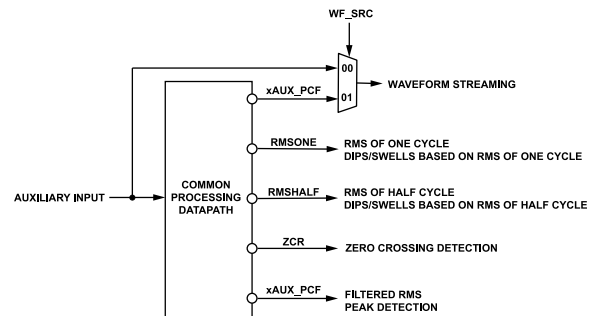
Figure 48. Auxiliary-Channel Datapath
