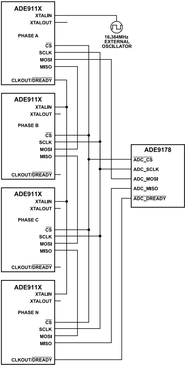
Figure 30. Four ADCs Connection Diagram to ADE9178
