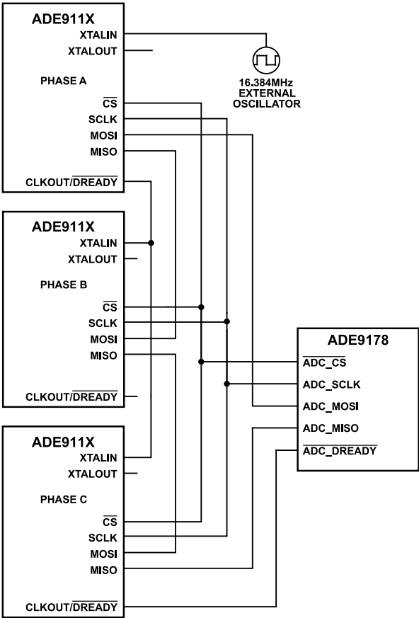
Figure 31. Three ADCs Connection Diagram to ADE9178
