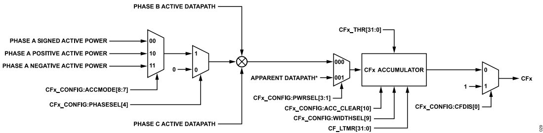
Figure 56. CF Pulse Active Datapath
