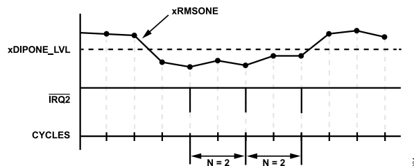
Figure 61. Continuous IRQ Mode
