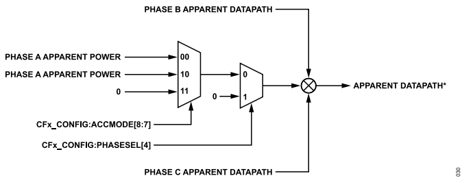
Figure 57. Apparent Datapath
