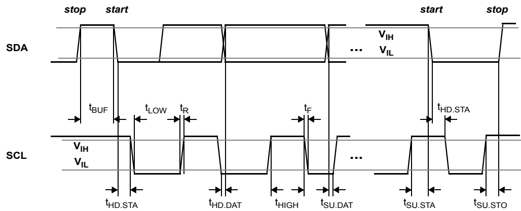
Figure 15. I 2 C timing characteristics
