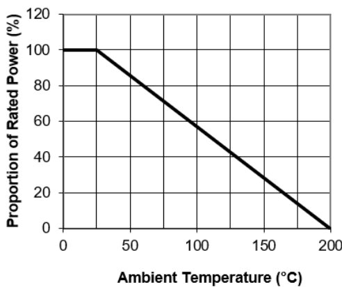
Derating for Ambient Temperature
