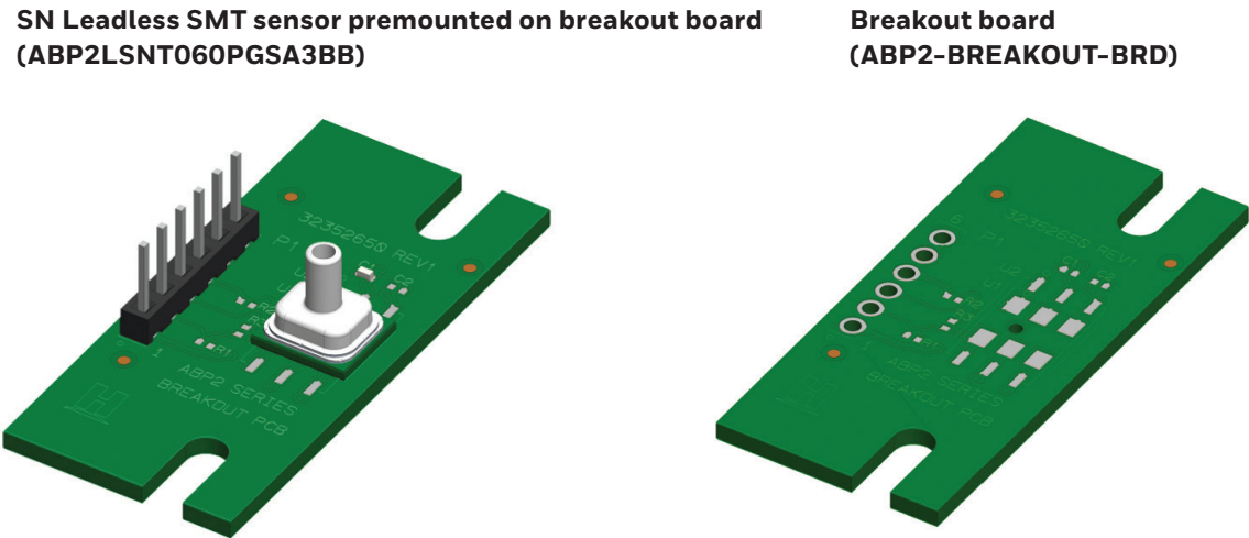
Figure 8. APB2 Series Sensors and Breakout Boards
