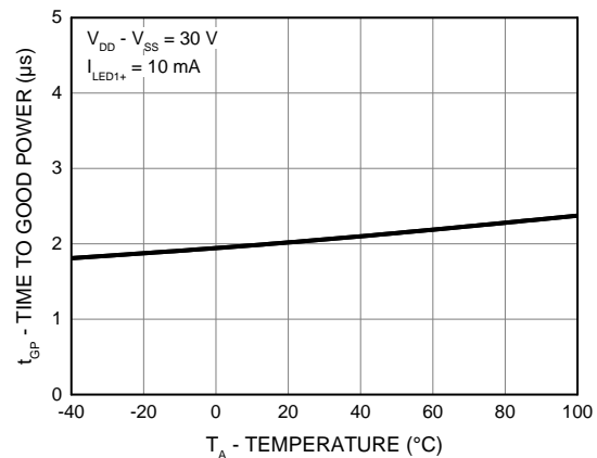
Figure 28. Time to Good Power ( t_{\text{GP}} ) vs. Temperature
