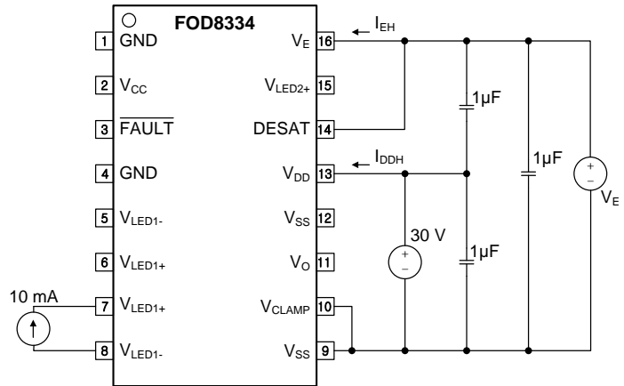
Figure 37. High Level Supply Current ( I_{DDH} ), V_E High Level Supply Current ( I_{EH} ) Test Circuit
