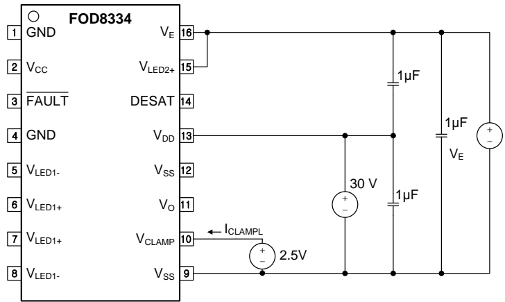
Figure 42. Clamp Low Sinking Current ( I_{CLAMP} ) Test Circuit
