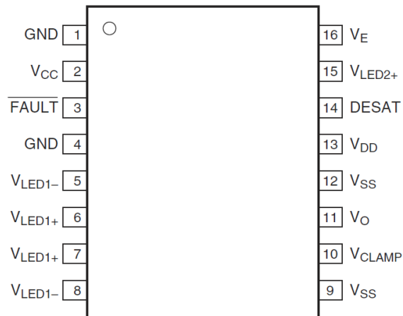
Figure 1. Pin Configuration
