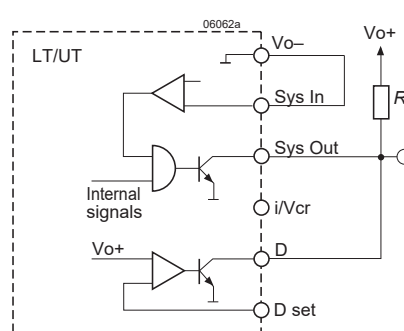
Fig. 30 Sys out and D connected in parallel.
