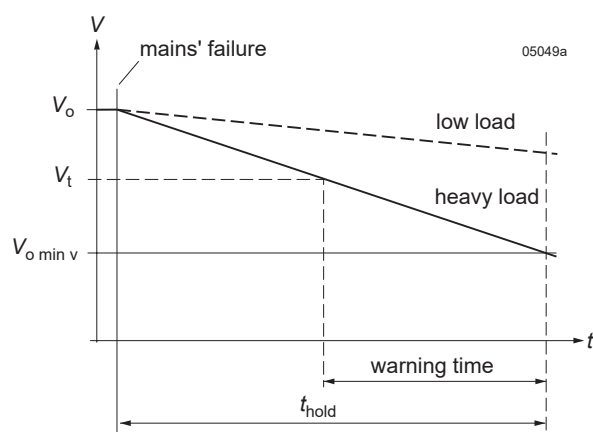
Fig. 15 Hold-up and warning time with Power Down output signal.
