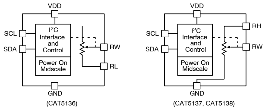
Figure 1. Block Diagram
