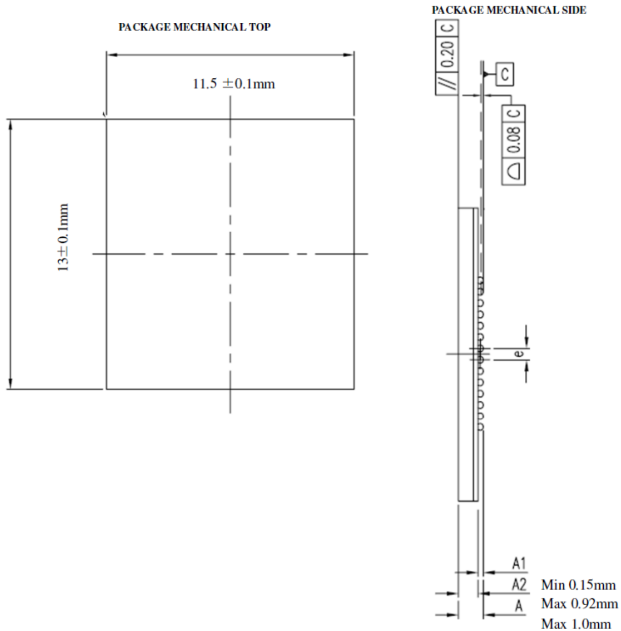
Figure 2 – Package Dimensions
