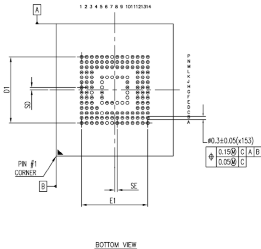
Figure 3 – Ball Pattern Dimensions
