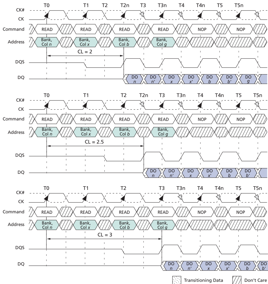
Figure 31: Random READ Accesses
