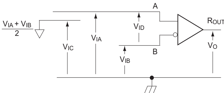
Figure 2. Receiver Voltage Definitions
