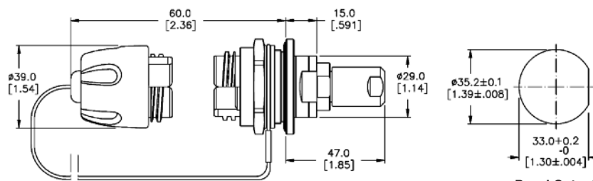
PRO BEAM Sr. D-Hole Bulkhead Connector with Standard Cable Adapter
