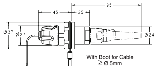
PRO BEAM Jr. Standard Bulkhead Connector, with Boot
