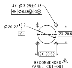
38999 Receptacle Shell Kit Wall Mount Flange
