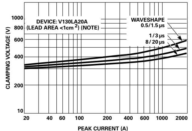
FIGURE 19A. V-I CHARACTERISTICS FOR VARIOUS CURRENT RISE TIMES
