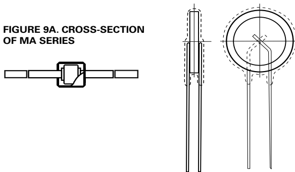
FIGURE 9B. CROSS-SECTION OF RADIAL LEAD PACKAGE
