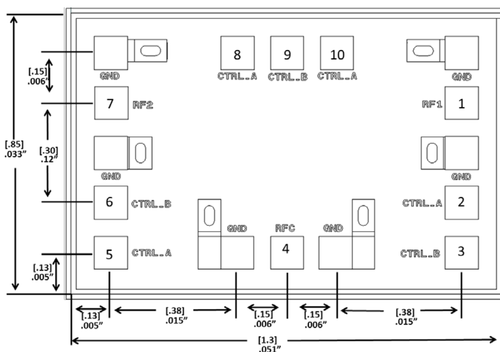
Figure 7 Chip Outline
