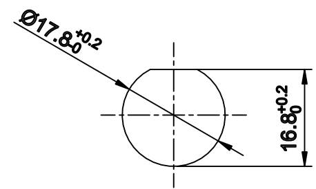
RECOMMEND MOUNTING HOLE
