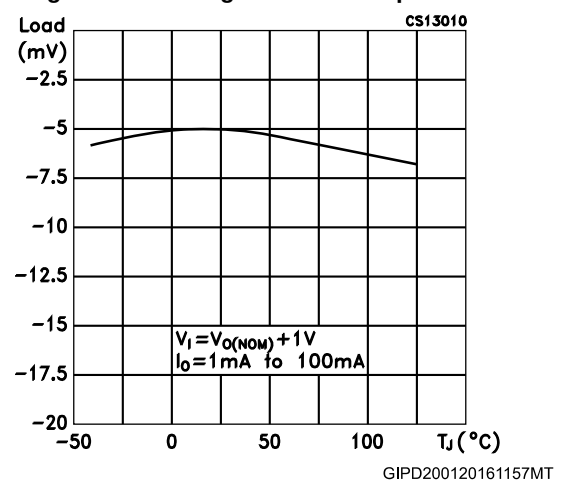
Figure 7: Load regulation vs temperature
