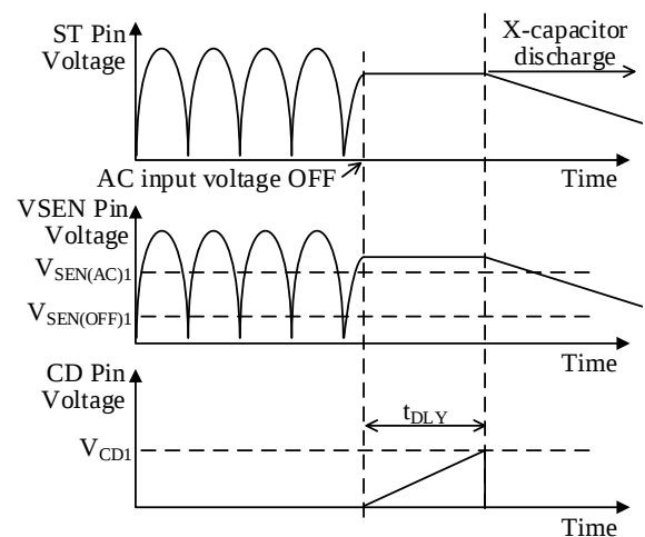
Figure 8-36. Operational Waveform of X-capacitor Discharge Function
