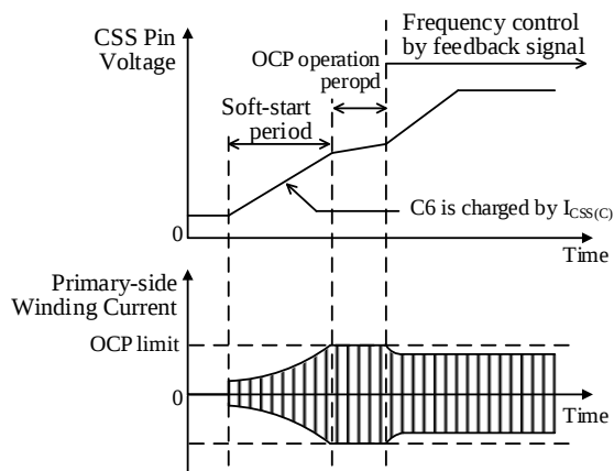
Figure 8-17. Soft-start Operation
