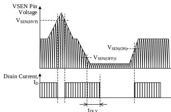
Figure 8-41. Input Voltage Detection Function Operational Waveforms
