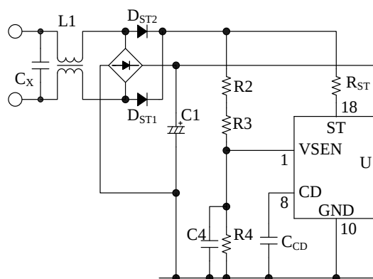
Figure 8-40. VSEN Pin Peripheral Circuit
