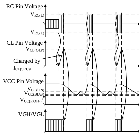
Figure 8-43. OLP Waveform
