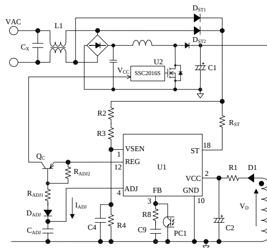
Figure 8-11. VCC Pin Peripheral Circuit When PFC ON/OFF Function is Enabled
