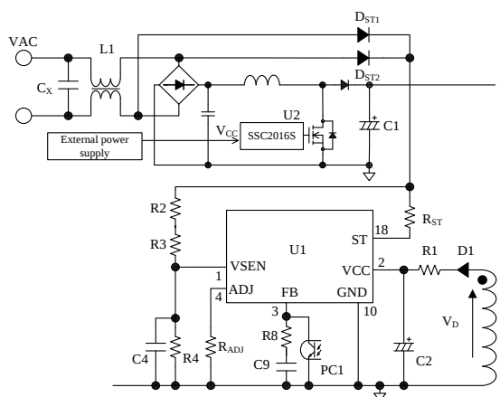
Figure 8-13. VCC Pin Peripheral Circuit When PFC ON/OFF Function is Disabled
