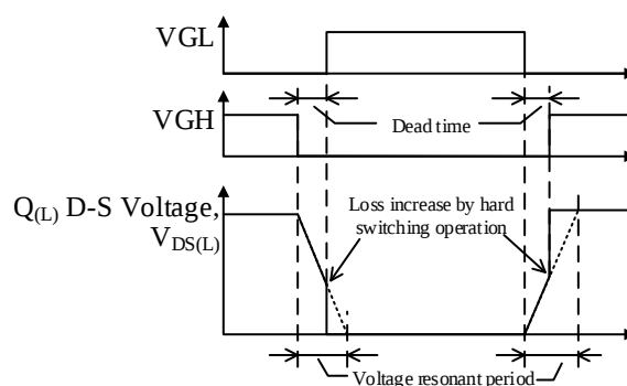
Figure 8-27. ZVS Failure Operation Waveform
