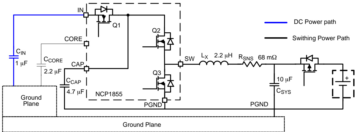
Figure 11. Power Path
