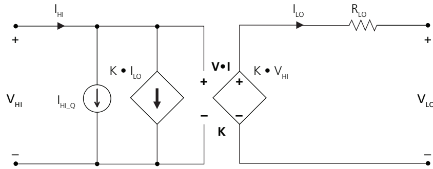
Figure 19 — BCM DC model (Forward Direction)
