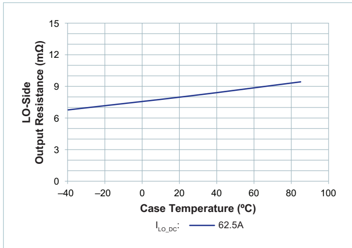
Figure 12 — R_{LO} vs. temperature; nominal V_{HI\_DC} I_{LO\_DC} = 62.5\text{A} at T_{CASE} = 85^{\circ}\text{C}
