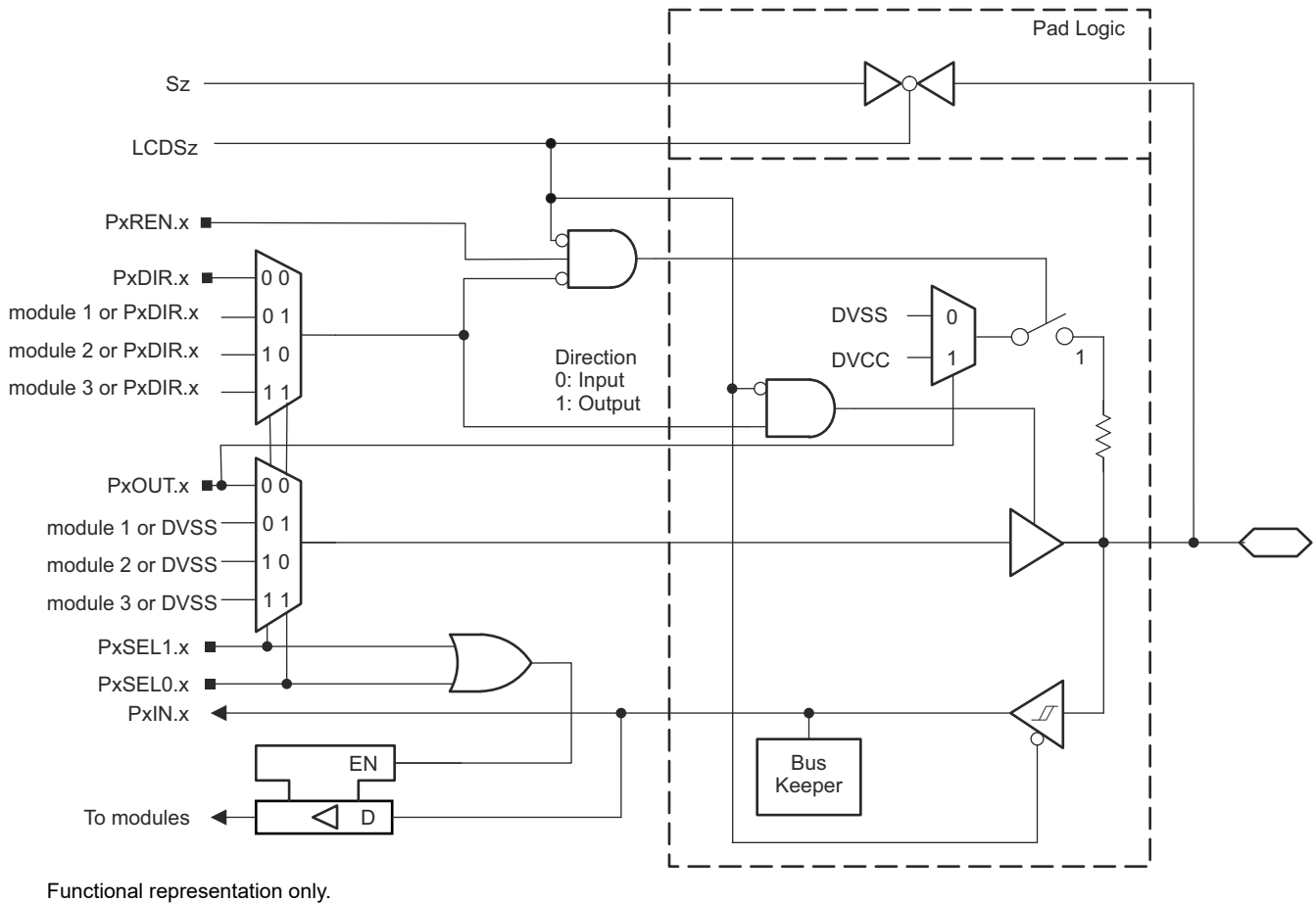
Figure 9-6. Port P2 (P2.4 to P2.7) Diagram
