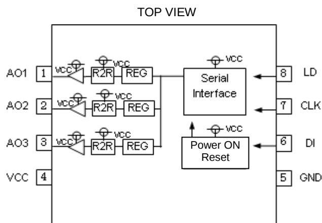
Figure 2. BH2220FVM
