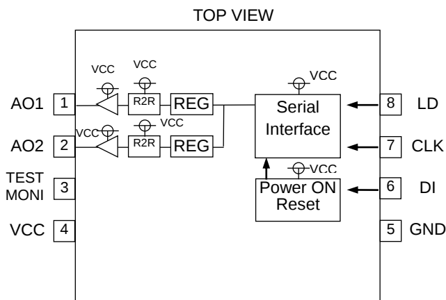
Figure 1. BH2219FVM
