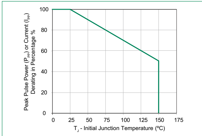
Peak Pulse Power Derating Curve
