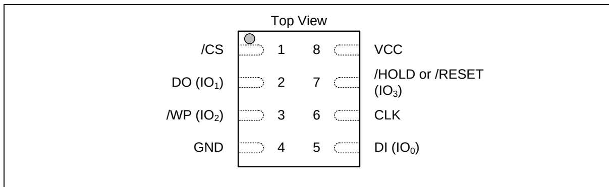
Figure 1b. W25Q128JW Pad Assignments, 8-pad WSON 6x5 (Package Code P / E )
