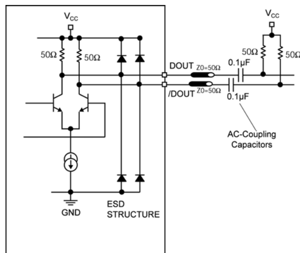
Figure 3. Output Structure
