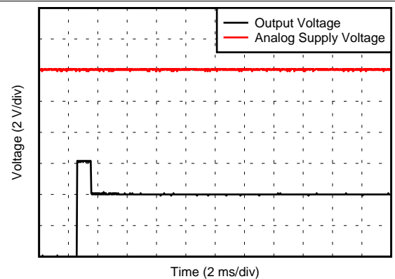
Figure 24. Output Response to a General-Call Reset
