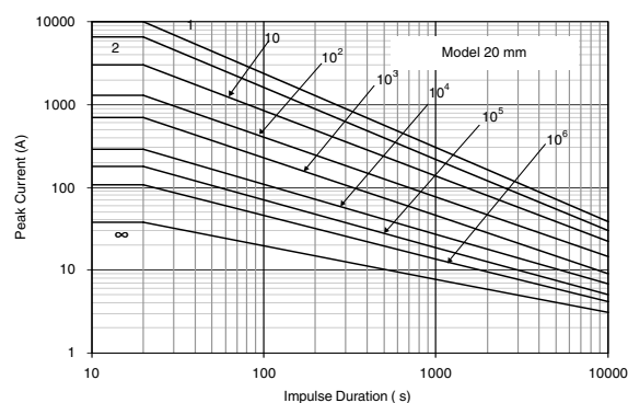
Figure 9: Pulse Rating Curves for 20mm types
