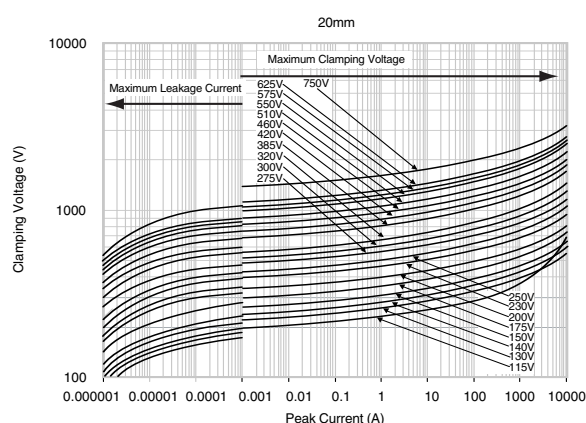
Figure 7: V-I Characteristic Curves for 20mm Types
